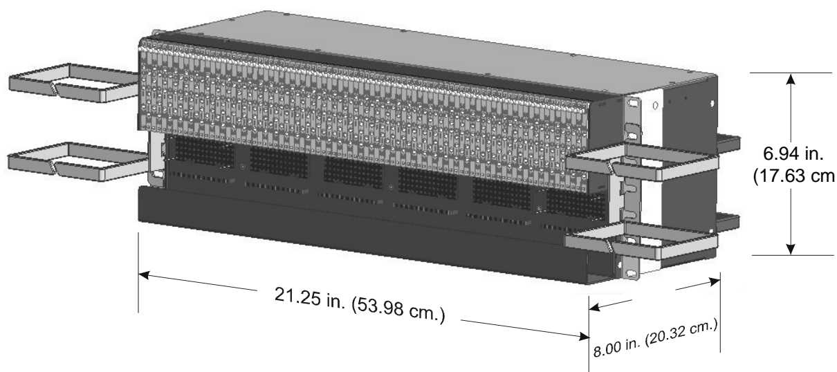
Figure 3 - Physical dimensions
