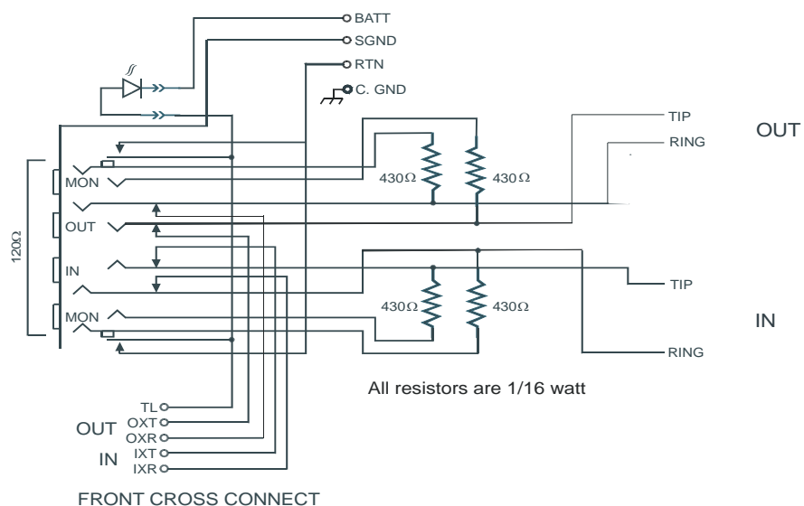
Figure 4 - Jack Schematic
