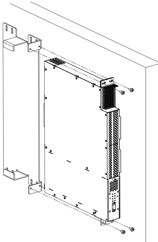
Figure 2 - Mounting on a wall
